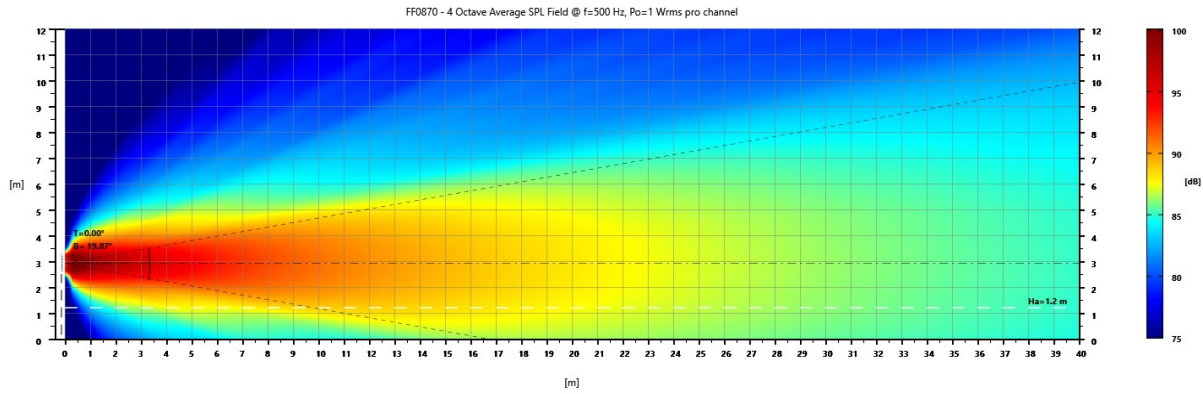
FF0870 – Vertical Beam Shape at 500 Hz, 4 Octaves average
