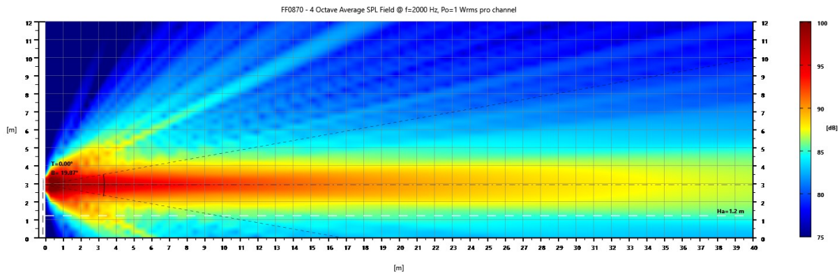
FF0870 – Vertical Beam Shape at 2000 Hz, 4 Octaves average
