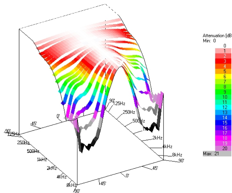
AH1635 - Horizontal Polar Responses vs Frequency
